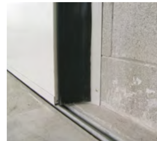
Guida inferiore incassata - Mod. Sliding with lower guide Lower guide - Mod. Sliding with lower guide
